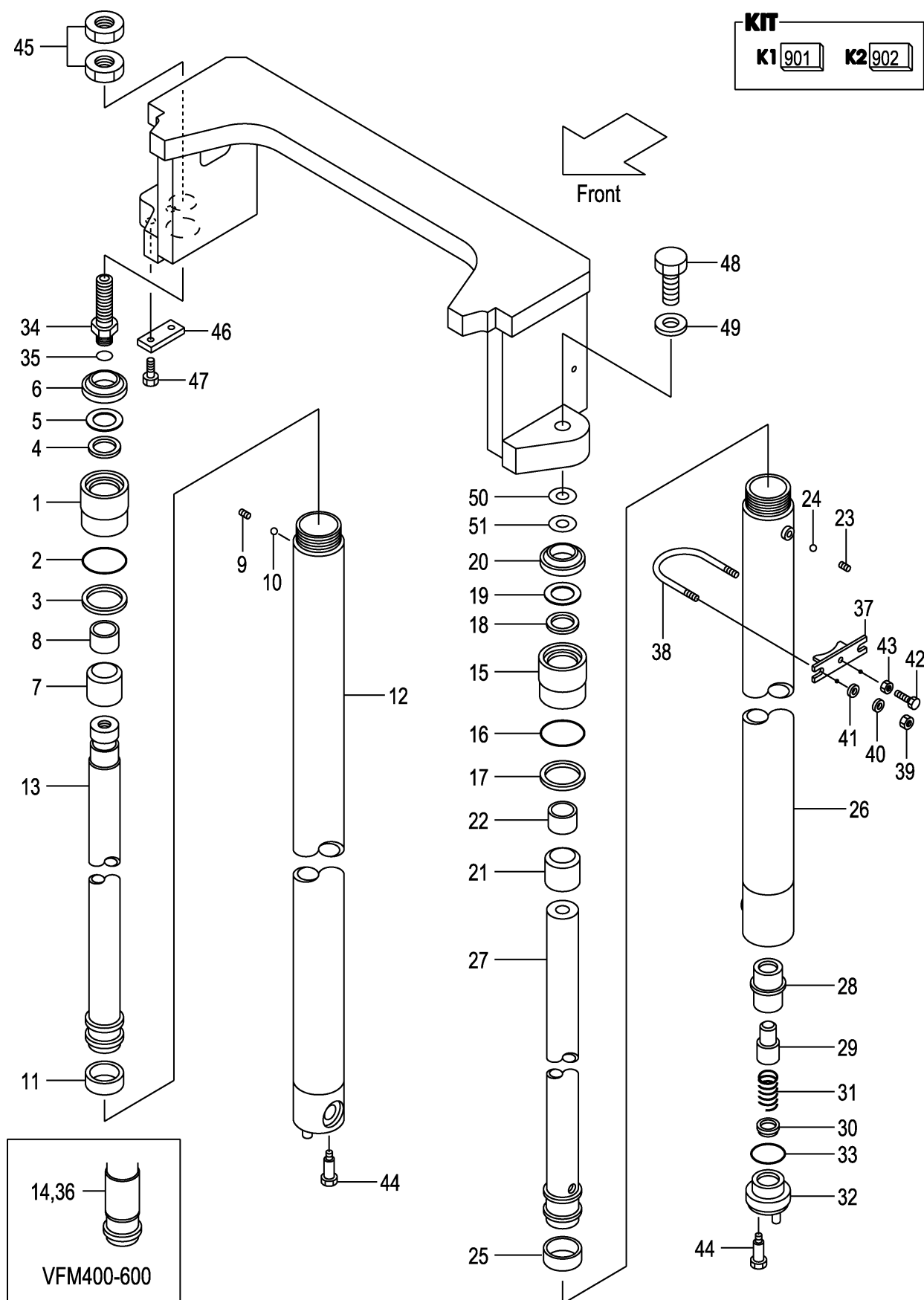
FIG.165 LIFT CYLINDER (REAR) [VFM2N9] (M7020550) リフトシリンダ(リヤ)
