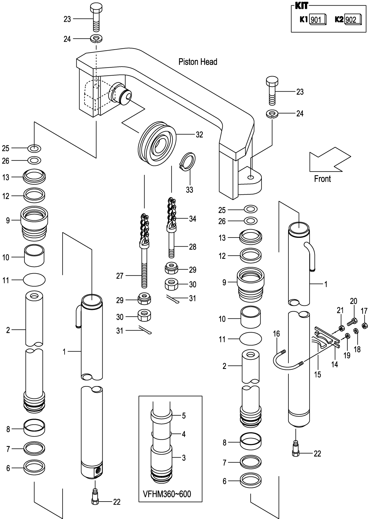
FIG.173 LIFT CYLINDER (REAR) [VFHM2N9] (M7020880) リフトシリンダ(リヤ)
